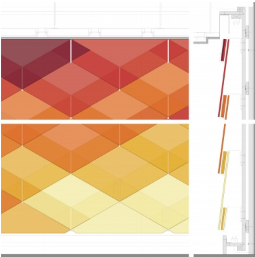
Detail Schindelwand
